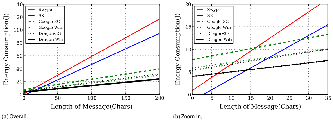
Fig. 9. Error corrected energy consumption comparison of three input modalities.
