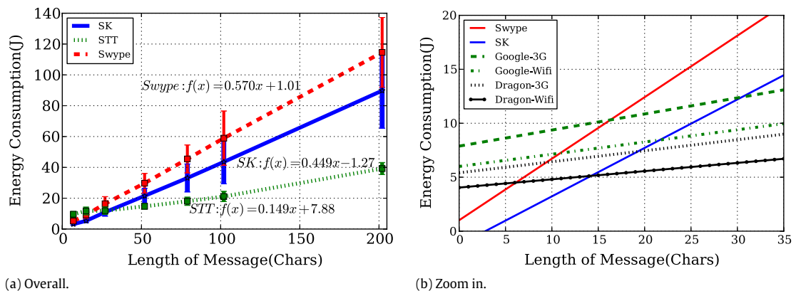
Fig. 4. Energy consumption comparison of three input modalities.
