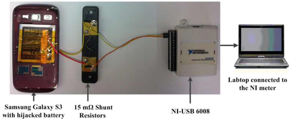
Fig. 1. Power measurement setup.
